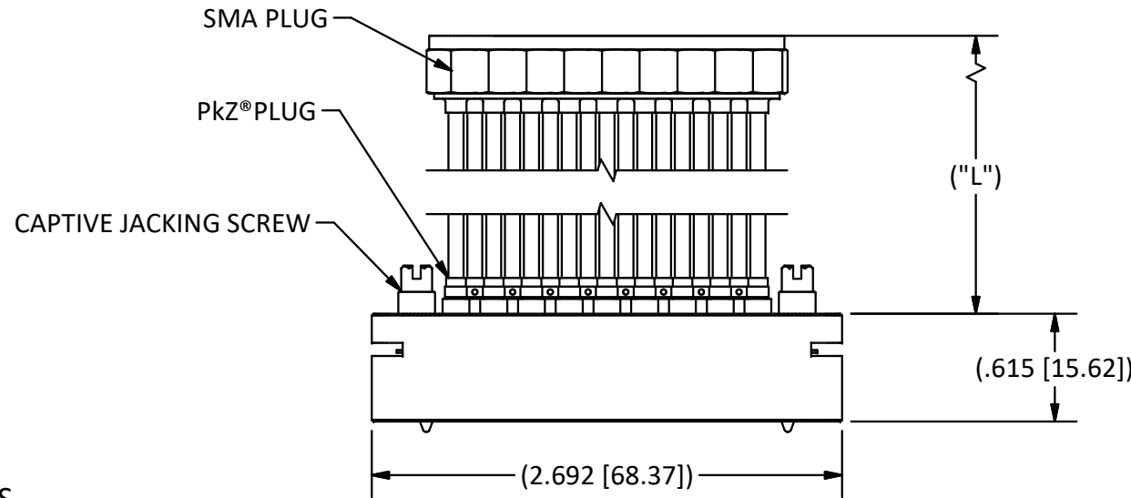
PART NUMBER HDQP03100-0201 SHOWN SCALE 1 : 1
