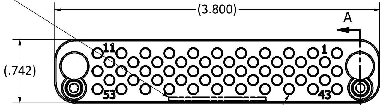
BACK VIEW
